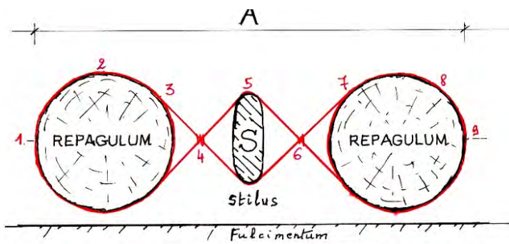
Fig. 28: Cross-section of Fig.27
