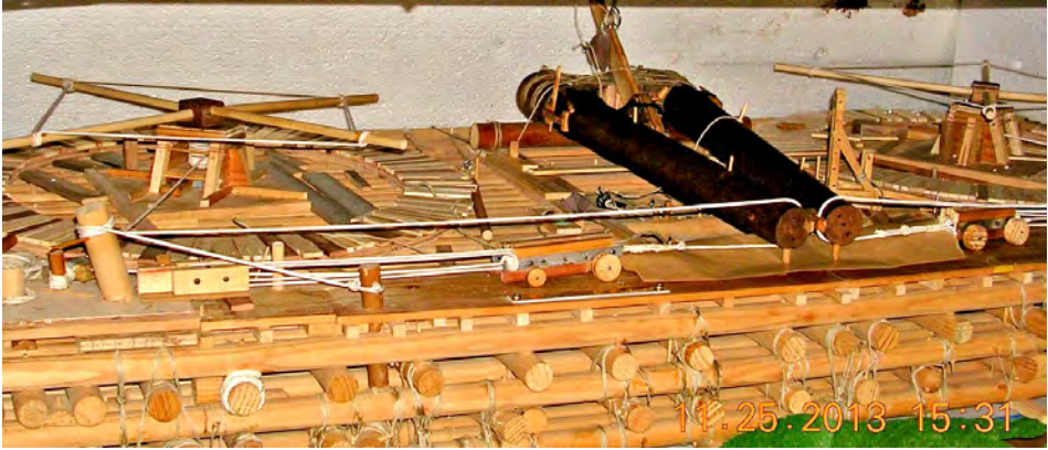
Fig. 29: A model of Version-2B, with the bogie-tackles upon the slide-table of the fulcimentum.
